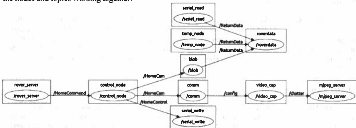
Figure 4 - Communication Paths
