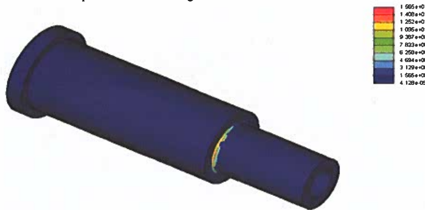
Figure 2 - FEA Suspension Pin
