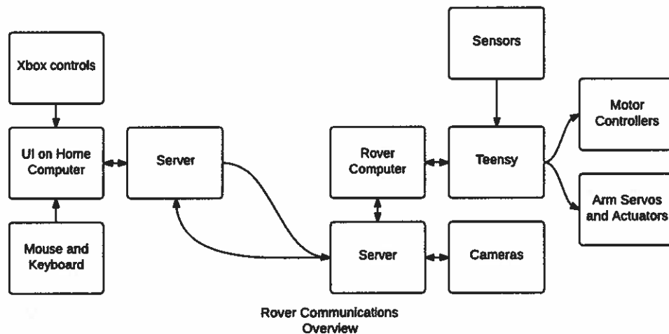
Figure 3 - Communication System
