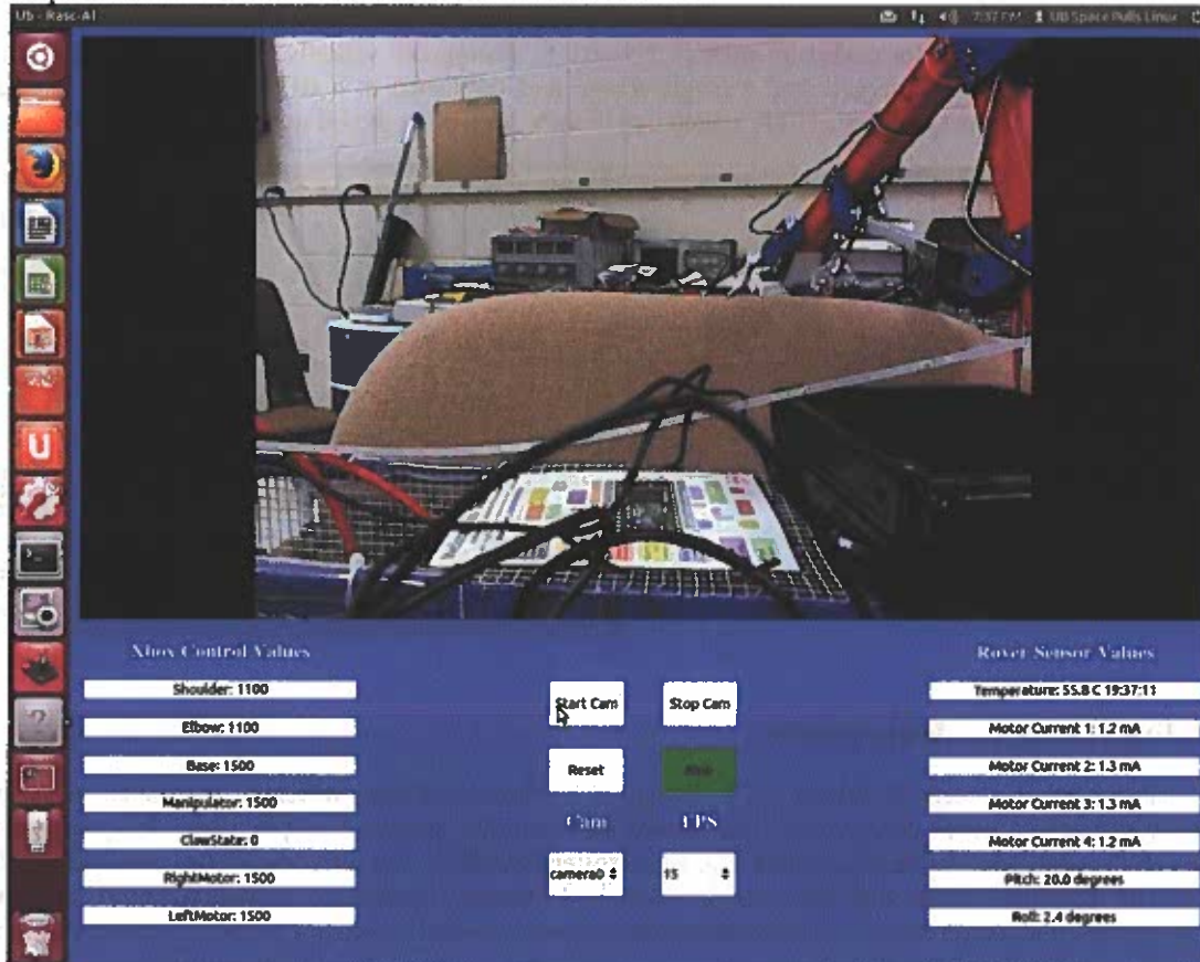
Figure 5 - User Interface
