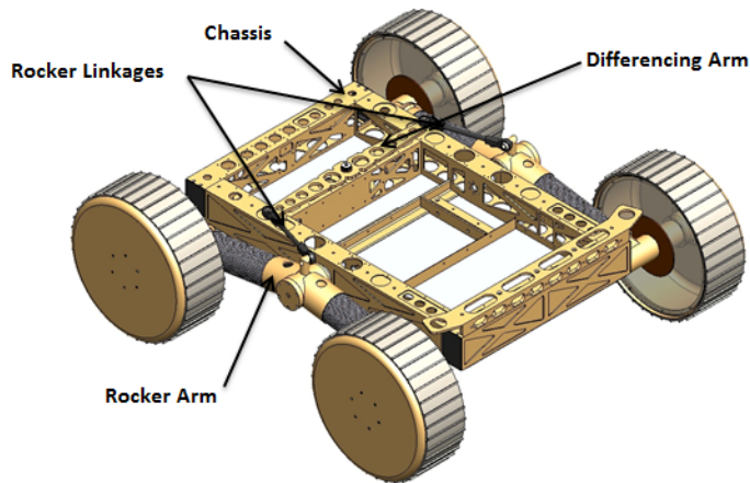
Figure 2: Chassis and Rocker Suspension Design
