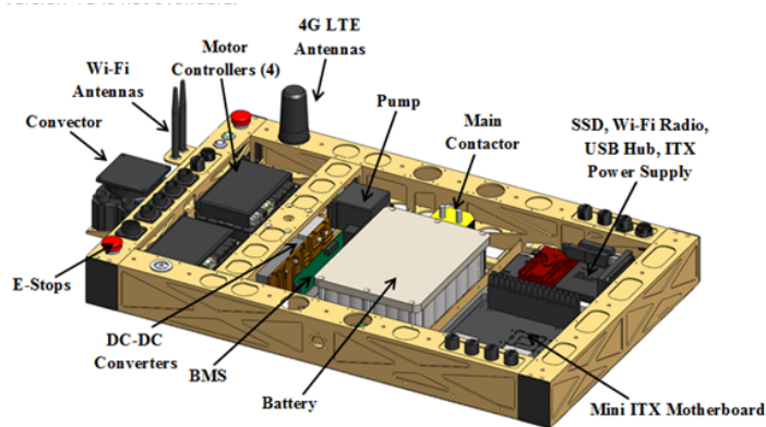
Figure 4 – internal components of ORYX 2.1
