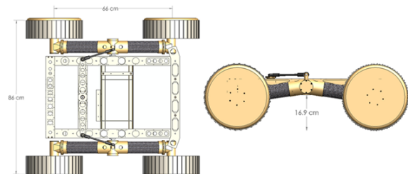
Figure 1 – Passive Averaging at Maximum and Rover Dimensions
