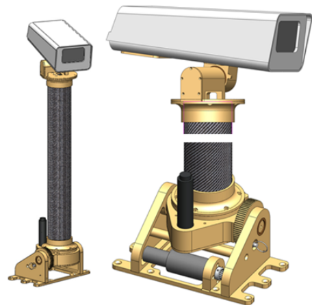
Figure 5 – pan-tilt camera on ORYX 2.1
