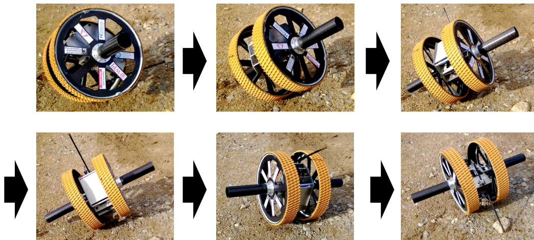
Figure 8- Micro-rover self-righting
